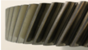
Nital edged gear with a thermal damage in the peripheral zone on the flanks of the teeth on the right.
